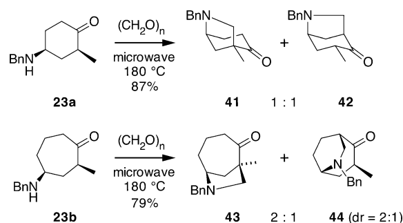
Scheme 6. Intramolecular Mannich reaction of 23 a and 23 b .
