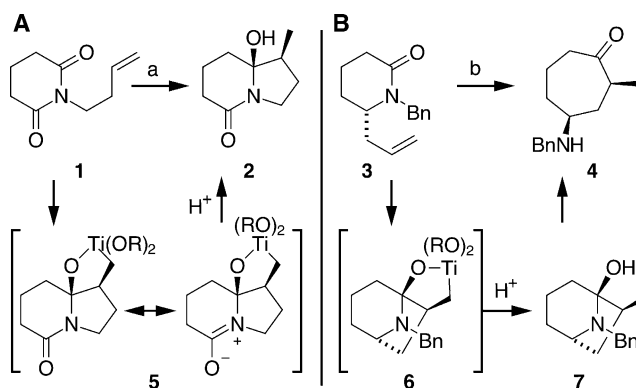
Scheme 2. Interrupted Kulinkovich–de Meijere reactions. A) Cha's imide substrates. [8] B) This work. Reagents and conditions: a) \text{ClTi}(\text{O}i\text{-Pr})_3 , c\text{-C}_5\text{H}_9\text{MgBr} , THF, rt, 44%; b) \text{Ti}(\text{O}i\text{-Pr})_4 , c\text{-C}_5\text{H}_9\text{MgBr} , THF, rt, 85%.
