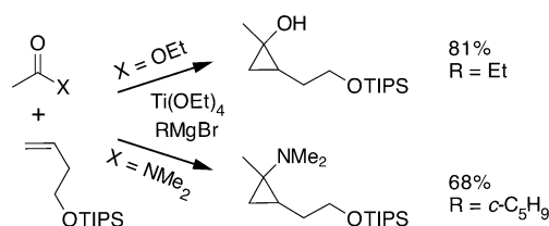
Scheme 1. Kulinkovich ( \text{X} = \text{OEt} ) and Kulinkovich–de Meijere ( \text{X} = \text{NMe}_2 ) reactions. [4]
