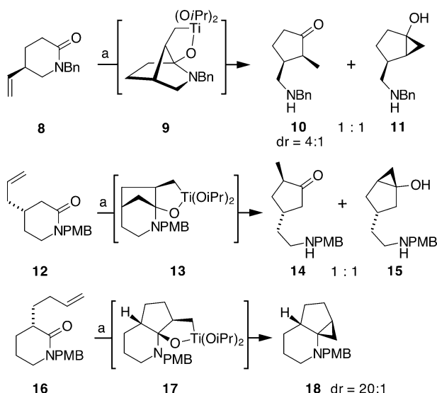
Scheme 3. Reaction of alkenes at other positions around the piperidinone. Reagents and conditions: a) \text{Ti}(\text{O}i\text{-Pr})_4 , c\text{-C}_5\text{H}_9\text{MgBr} , THF, rt, (33 % for 10 , 40 % for 14 + 15 , 73 % for 18 ).
