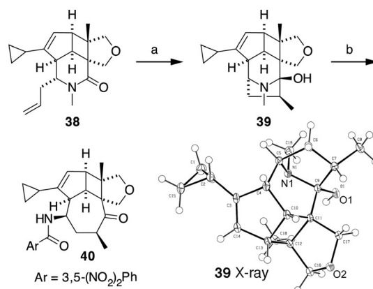
Scheme 5. Polycyclic substrate. Reagents and conditions: a) \text{Ti}(\text{O}i\text{-Pr})_4 , c\text{-C}_5\text{H}_9\text{MgBr} , THF, rt, 93%; b) 3,5-( \text{O}_2\text{N} ) _2\text{C}_6\text{H}_3\text{COCl} , \text{Et}_3\text{N} , 75%.
