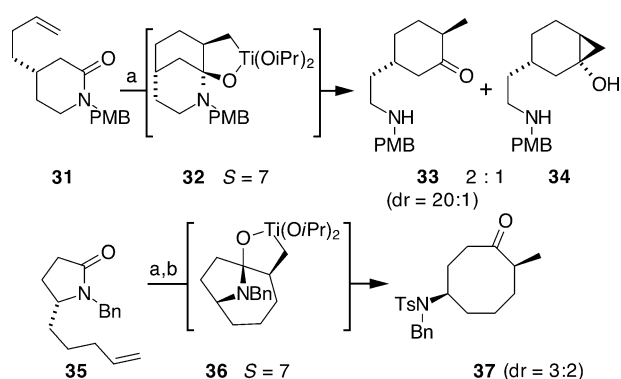
Scheme 4. Changes in side chain length. Reagents and conditions: a) \text{Ti}(\text{O}i\text{-Pr})_4 , c\text{-C}_5\text{H}_9\text{MgBr} , THF, rt, b) \text{TsCl} , pyridine (40% for 33 ; 27% for 37 as a 3:2 mixture of diastereomers).
